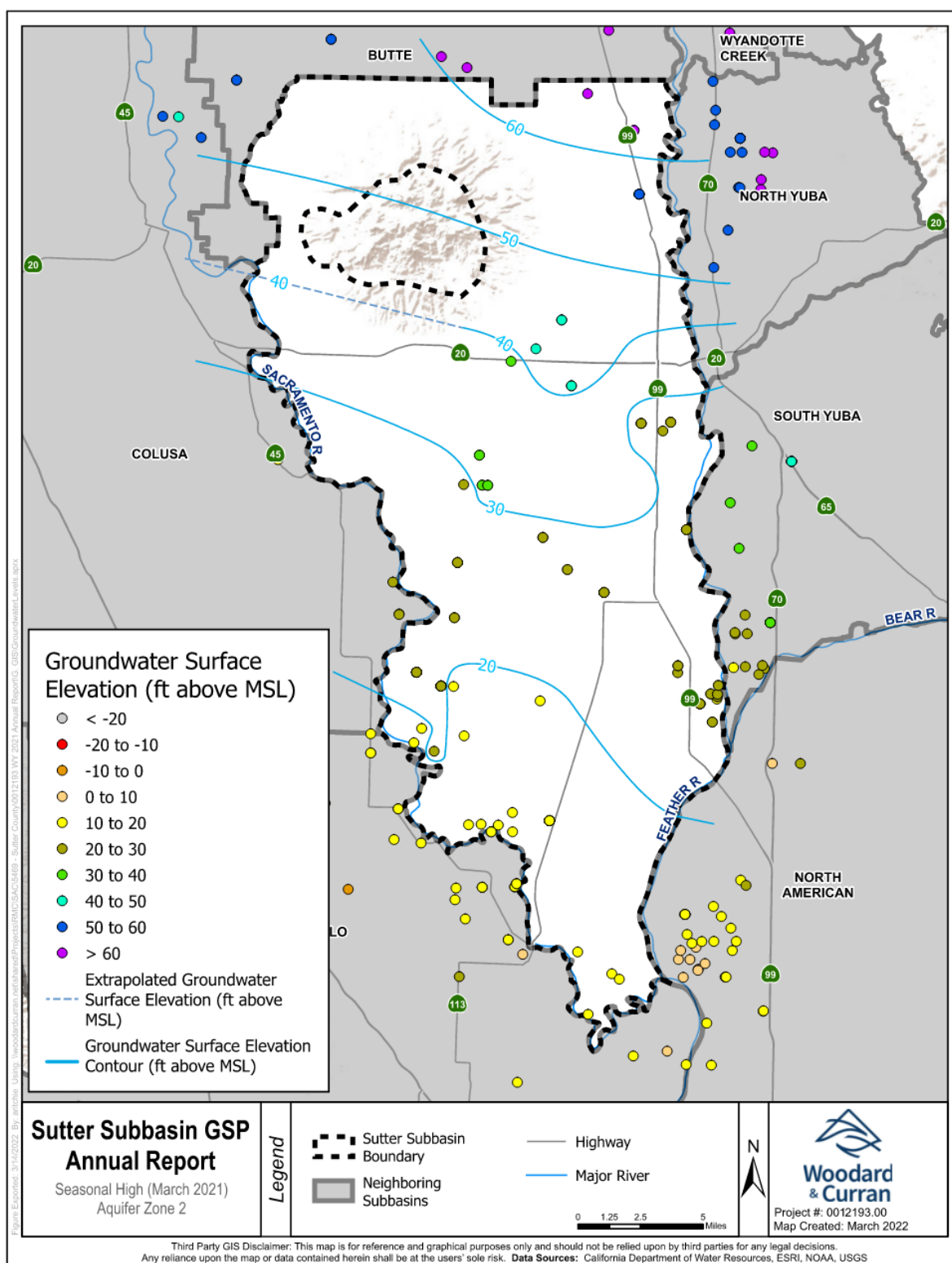
Figure 3-7: Seasonal High Groundwater Levels in AZ-2, March 2021
