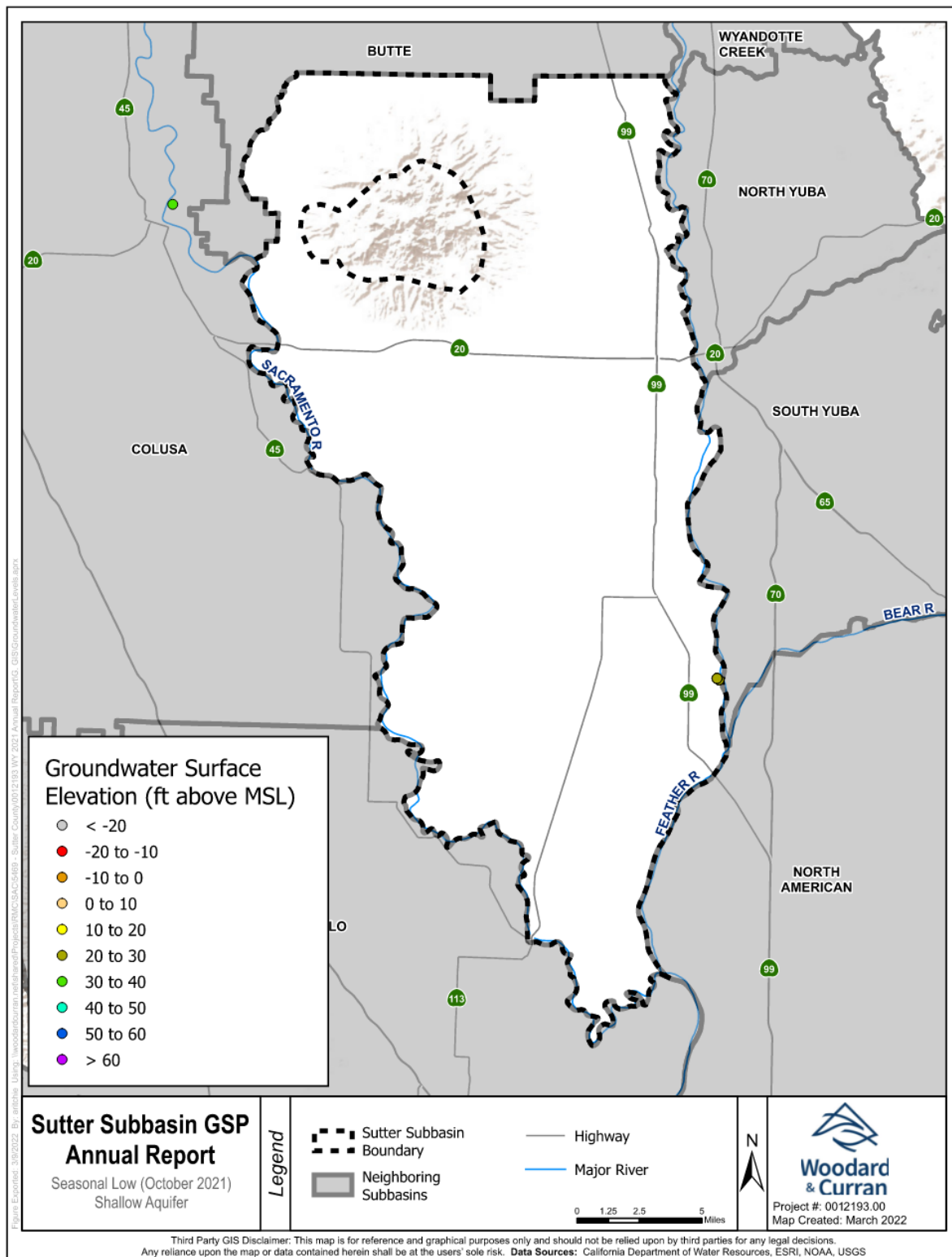
Figure 3-9: Seasonal Low Groundwater Levels in Shallow AZ, October 2021
