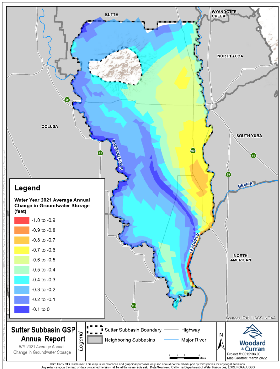
Figure 3-14: WY 2021 Change in Groundwater Storage
