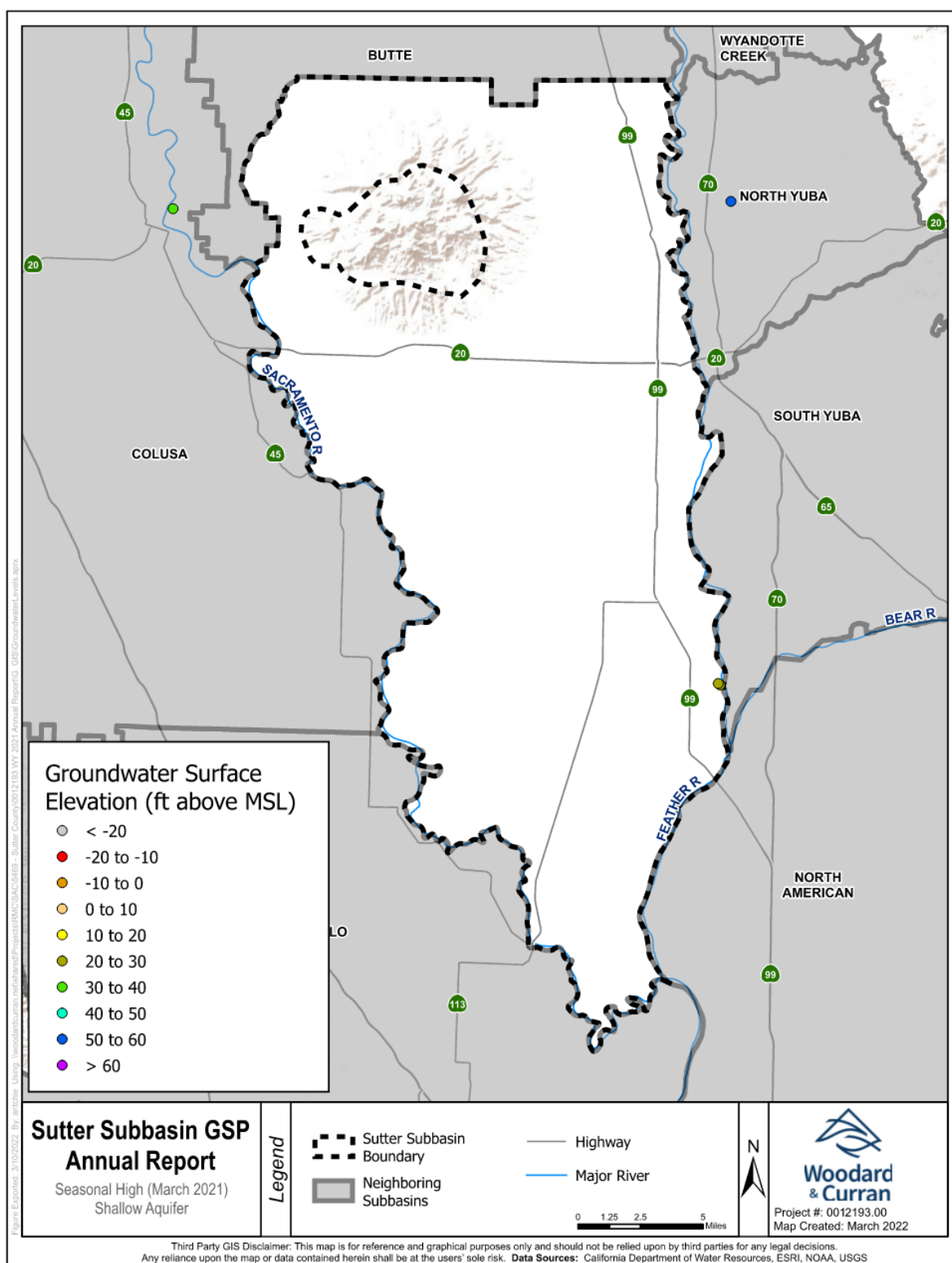
Figure 3-5: Seasonal High Groundwater Levels in Shallow AZ, March 2021
