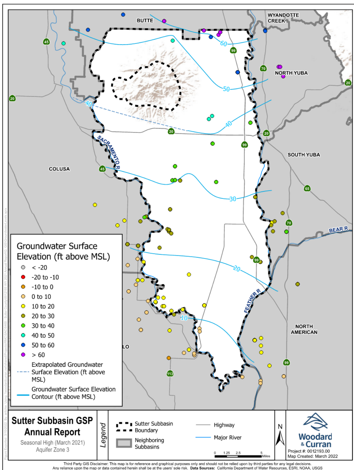
Figure 3-8: Seasonal High Groundwater Levels in AZ-3, March 2021
