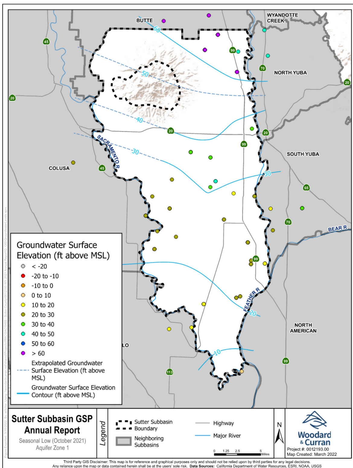
Figure 3-10: Seasonal Low Groundwater Levels in AZ-1, October 2021
