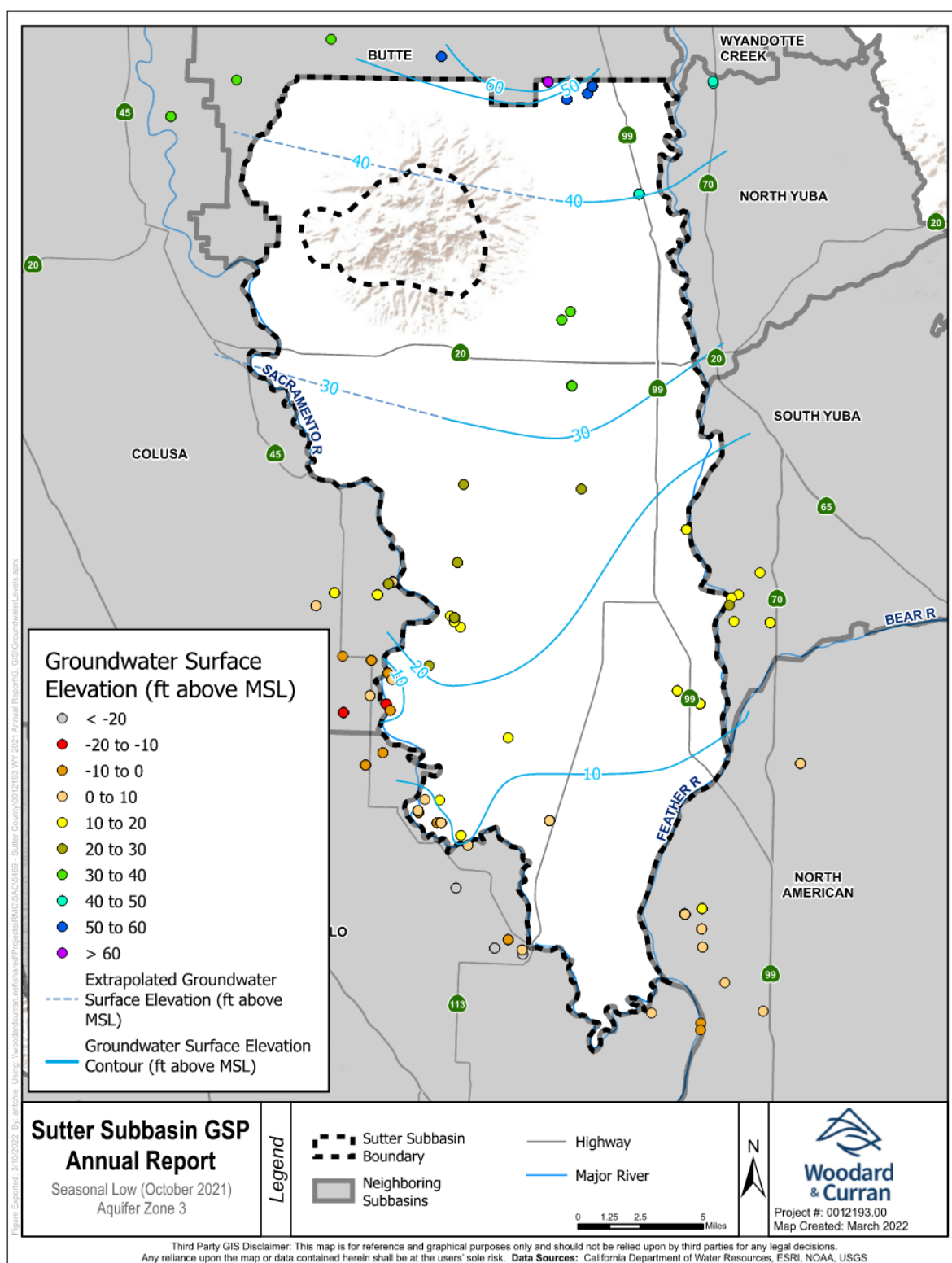
Figure 3-12: Seasonal Low Groundwater Levels in AZ-3, October 2021
