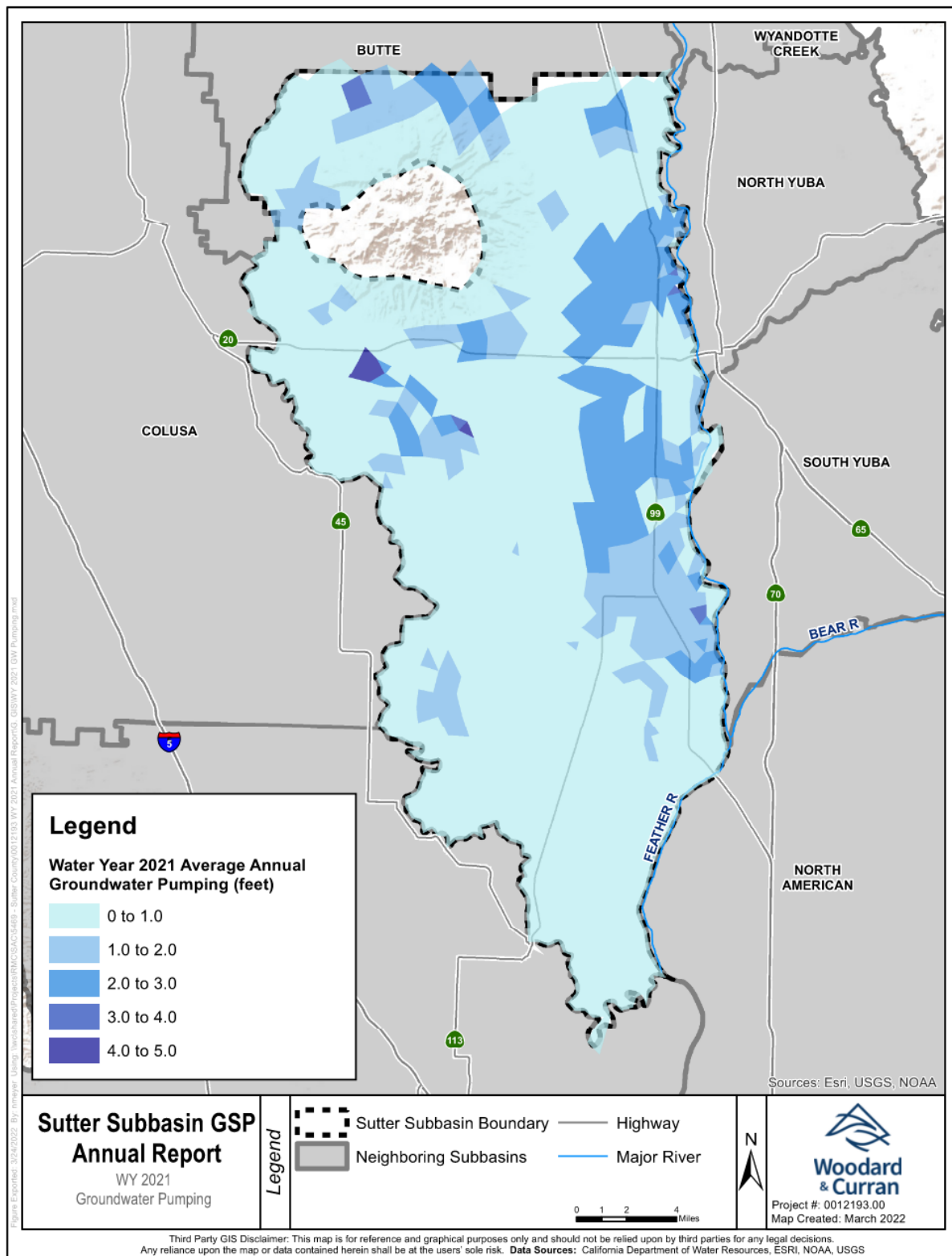
Figure 3-26: WY 2021 Groundwater Pumping
