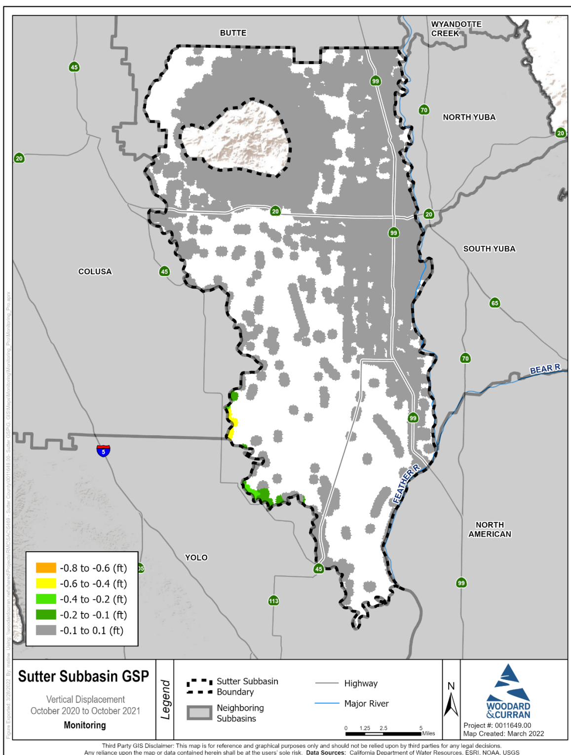
Figure 3-21: Vertical Displacement in the Sutter Subbasin, October 2020 to October 2021
