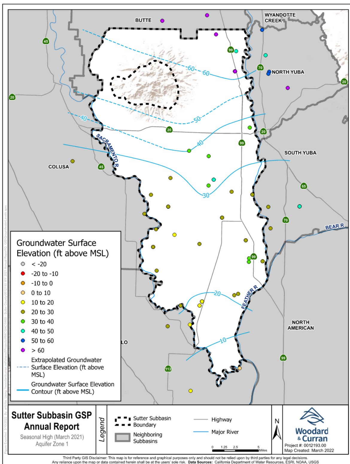
Figure 3-6: Seasonal High Groundwater Levels in AZ-1, March 2021
