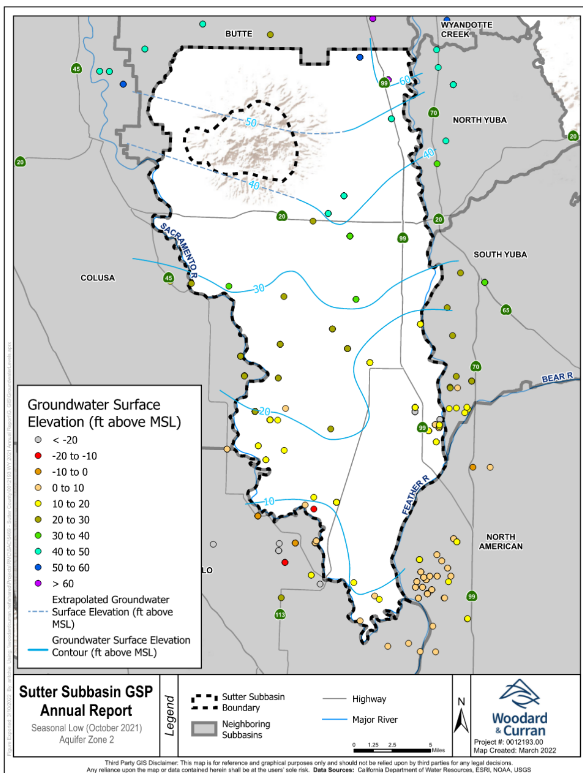
Figure 3-11: Seasonal Low Groundwater Levels in AZ-2, October 2021
